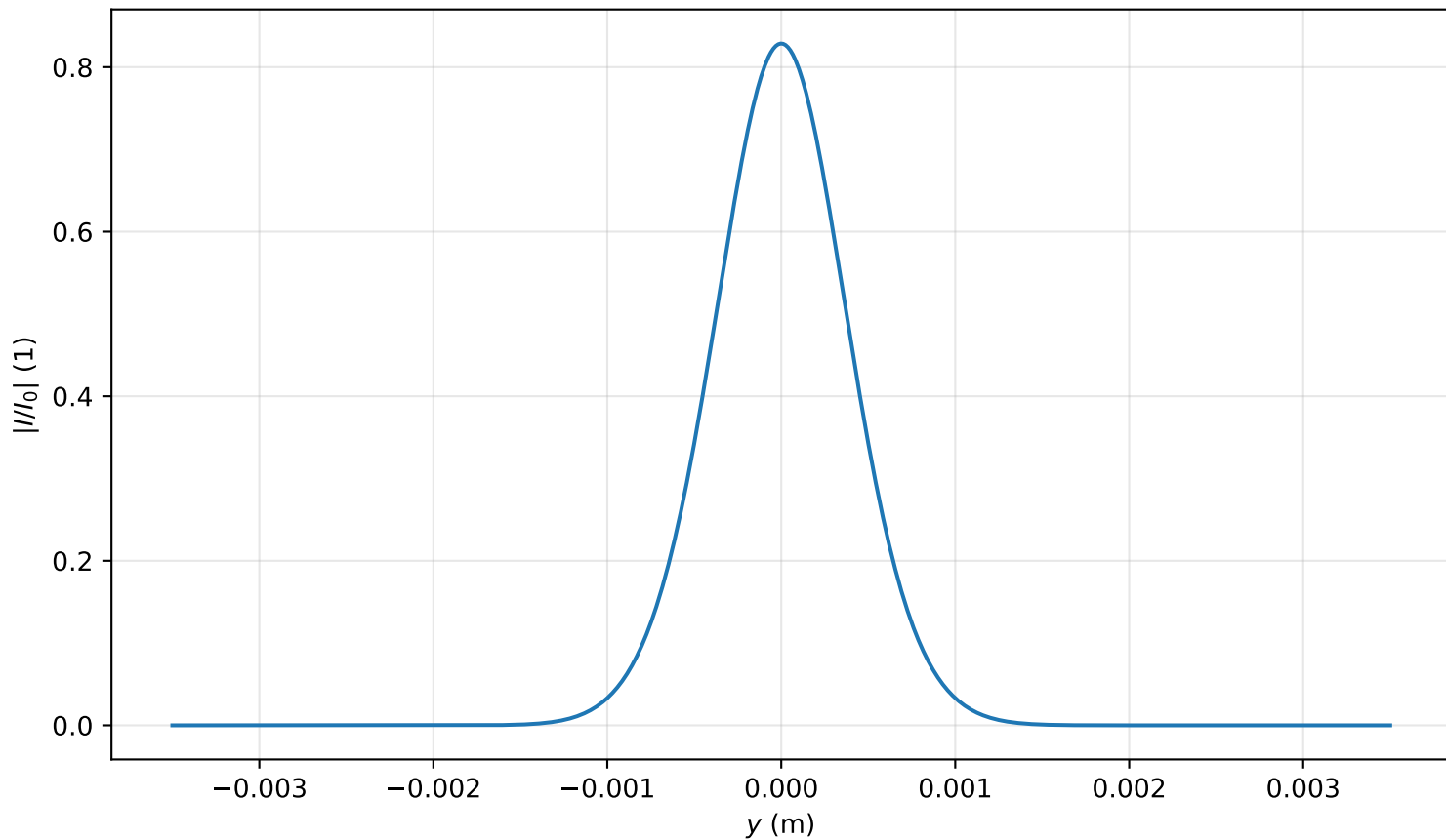
Intensity profile I(x=0, y, z=1.194)/I_0 , P_{in}=0.2P_{cr} , artificial time
